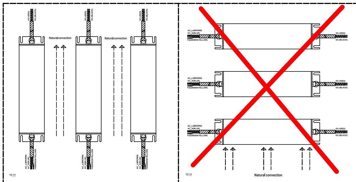
[Fig. 3] Installation method
