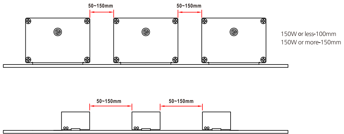
[Fig.1] Product installation spacing
